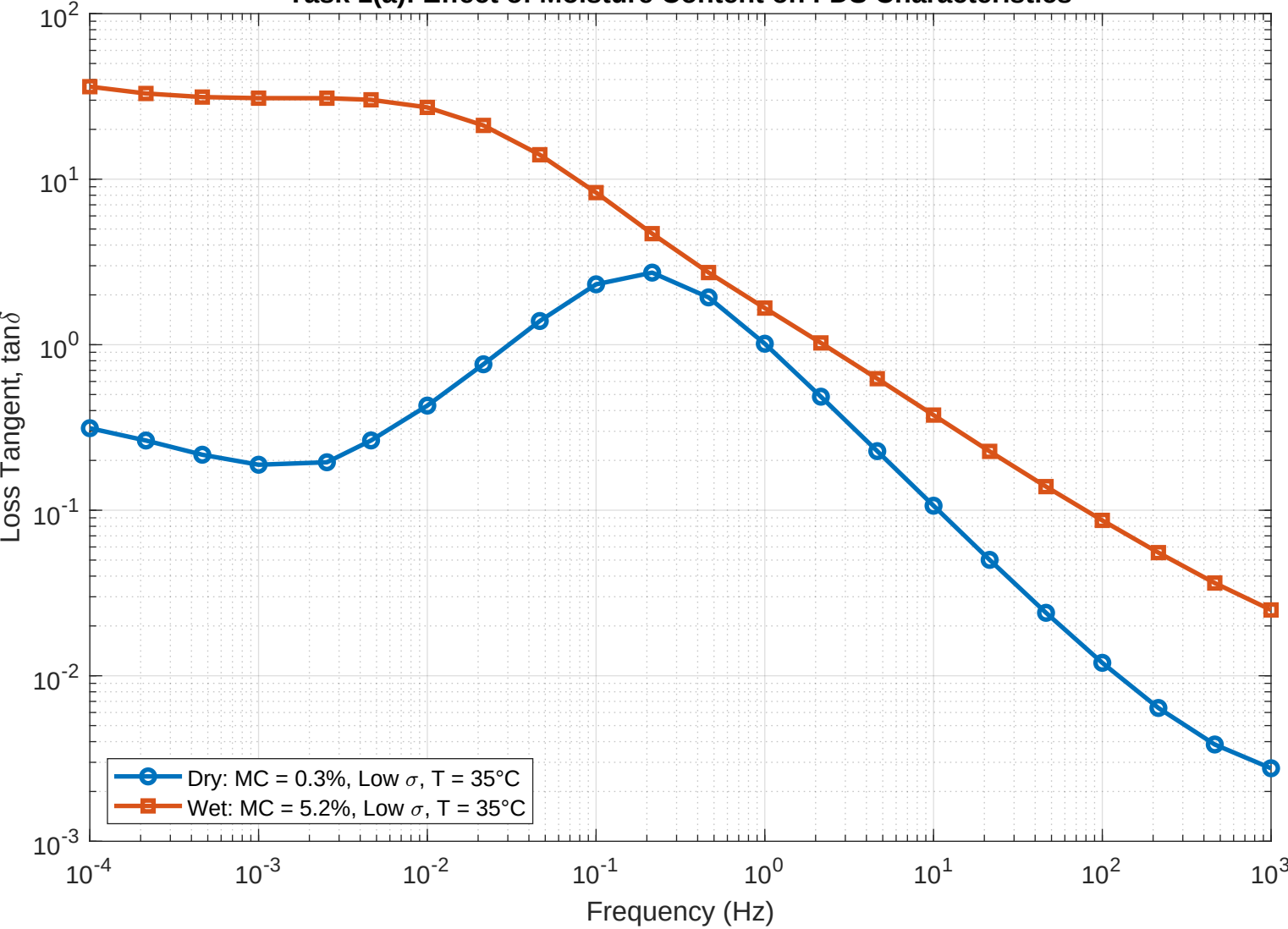
Task 1(a): Effect of Moisture Content on FDS Characteristics
